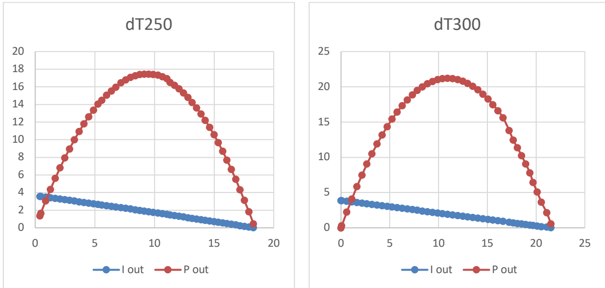
Figure 7 Individual plots for \Delta T = 50, 100, 150, 200, 250, 300 degrees Celsius. Voltage (V, Blue) and Power (W, Red) versus Current (A).
