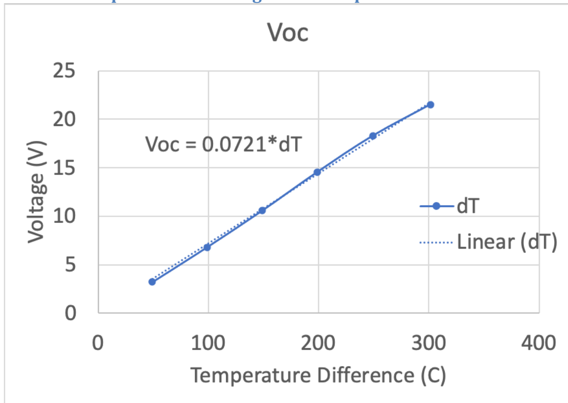
Figure 3 Open-circuit Voltage from the main circuit (Blue) vs temperature difference (°C). The mathematical relationship is also shown.
